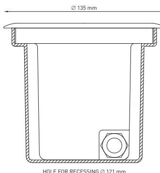
201015P HYDROFLOOR COMPACT SQUARE GU5.3
