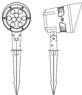
106004 HYDROSKY MEDIUM LED WITH EARTH SPIKE
