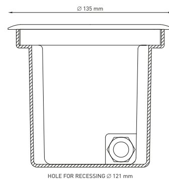
201018P HYDROFLOOR COMPACT SQUARE GU10
