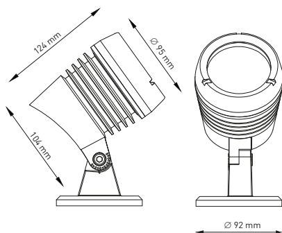
107005 HYDROJET MEDIUM LED WITH MOUNTING BASE
