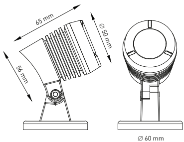
107001 HYDROJET MICRO LED WITH MOUNTING BASE
