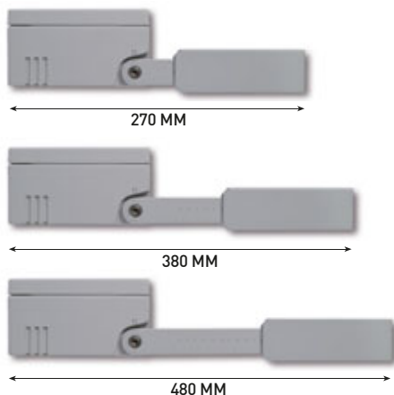
WATER DRAINAGE
