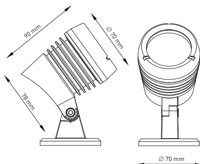
107003 HYDROJET MINI LED WITH MOUNTING BASE
