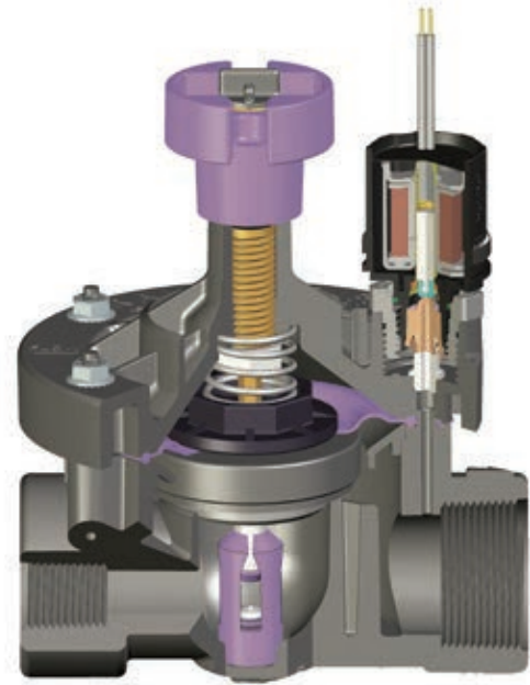
PESB-R Cutaway
